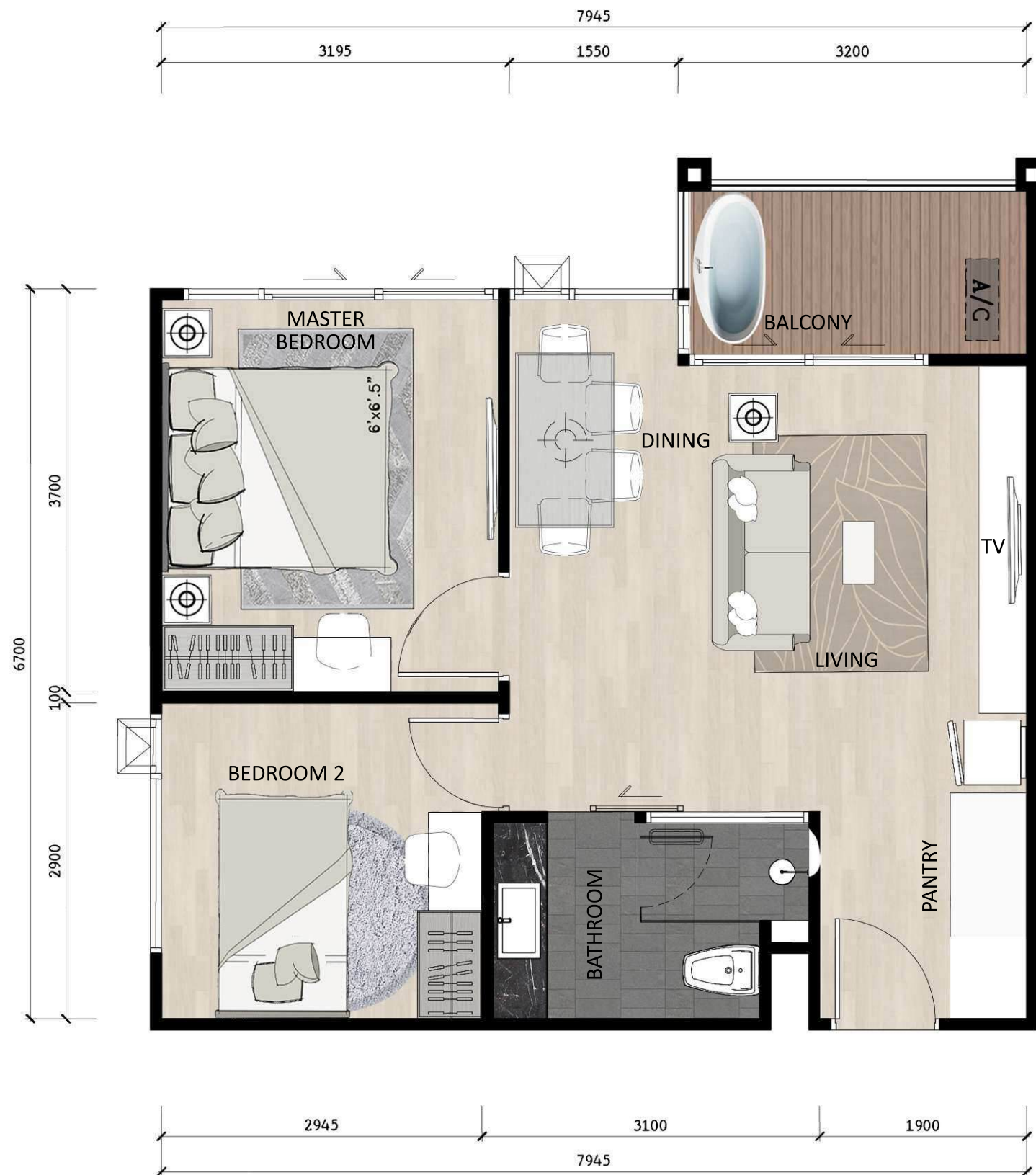
TYPE B 55.23 SQ.M.
