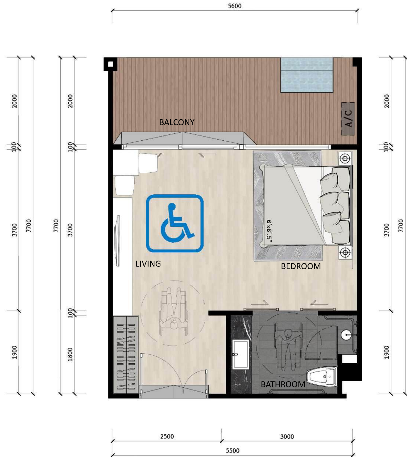
TYPE A1(HD) 43.59 SQ.M. POOL ACCESS
