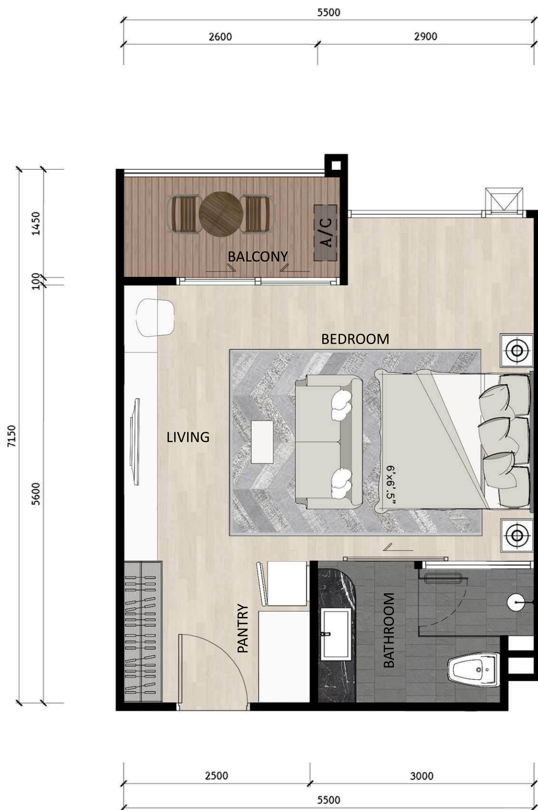
TYPE A5 34.97 SQ.M.
