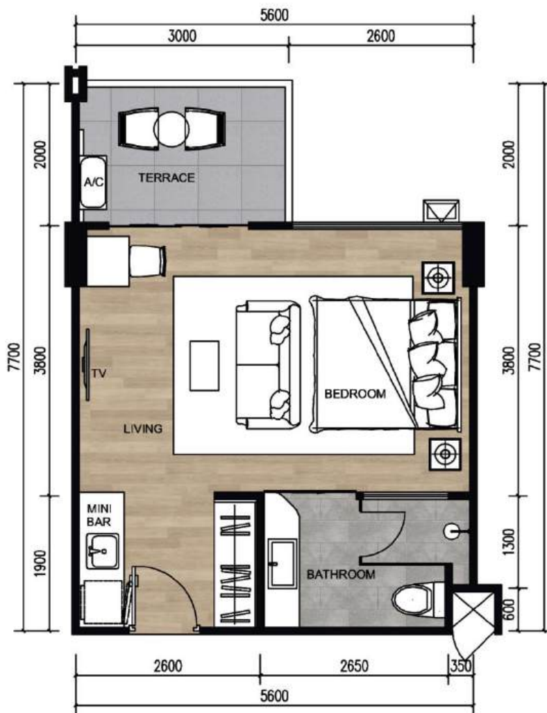
TYPE A+ 37.1 SQ.M.
